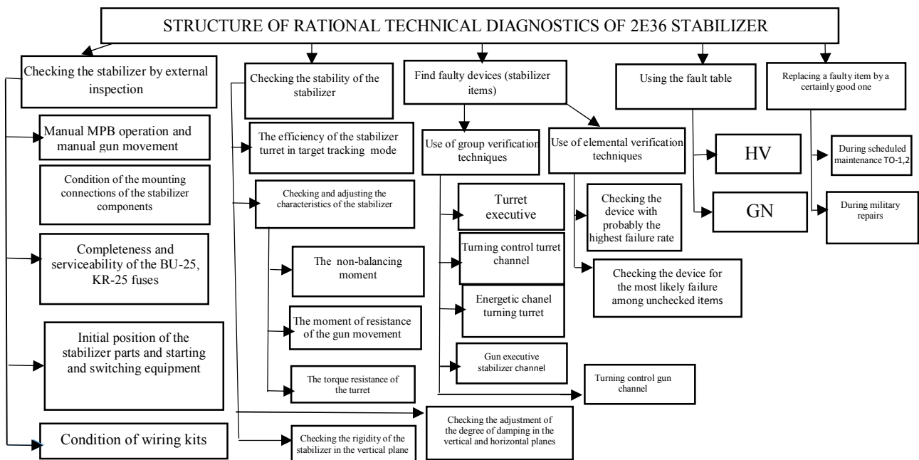
Fig. 3. Structure of rational technical diagnostics of 2E36 stabilizer
