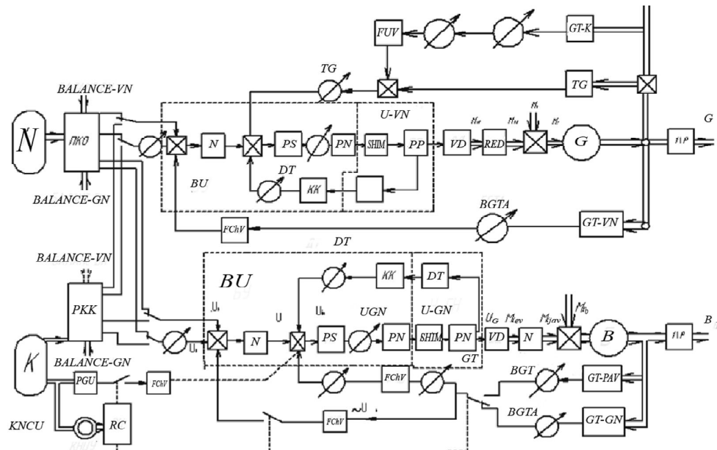
Fig. 1. Functional logic scheme of 2E36
